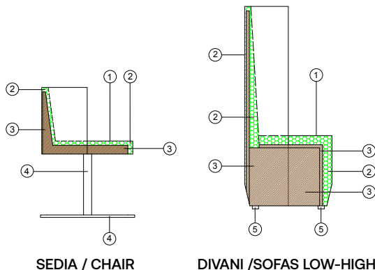
SEDIA / CHAIR
