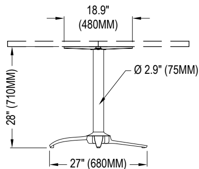
DINING ELEVATION
