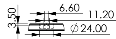
DETAIL B
