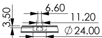
DETAIL A
